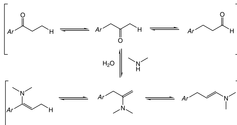
Fig. 2. Isomerization and the effect of water on enamines
