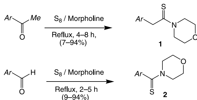
Fig. 1. The synthesis of terminal thioamides 1 and 2 under the WK reaction
