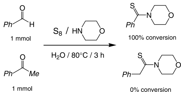
Fig. 3. Chemoselective thioamidation of benzaldehyde in the presence of acetophenone in water
